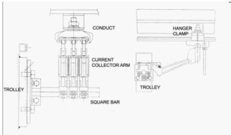
3 Phase Power rail
